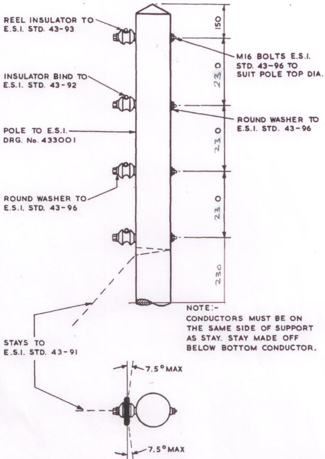
Fig. 2 Intermediate support (deviations up to 15°) (ESI Drawing 433002)
